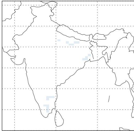
Change of Sulfate Due to Traffic: REF
