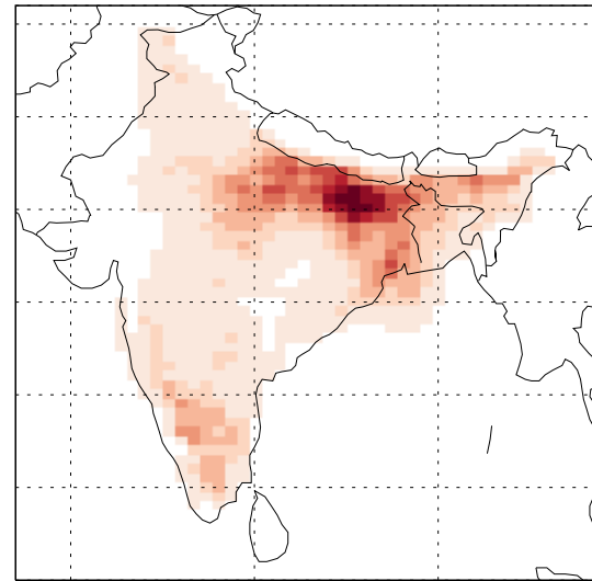
Change of Nitrate Due to Traffic: S2
