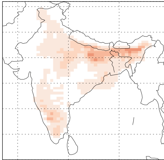
Change of Nitrate Due to Traffic: REF
