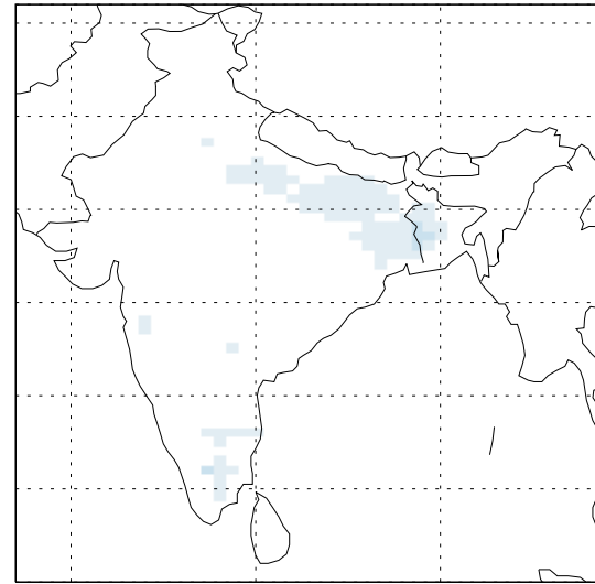
Change of Sulfate Due to Traffic: S2
