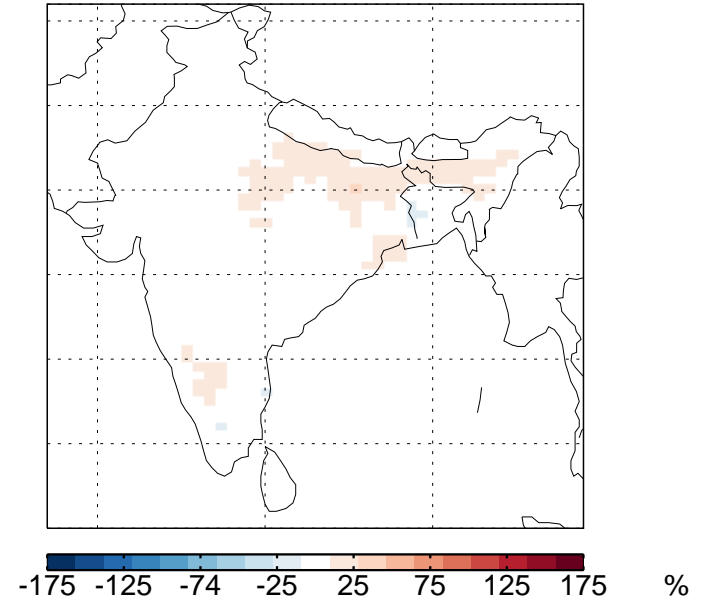
Change of Ammonium Due to Traffic: S2
