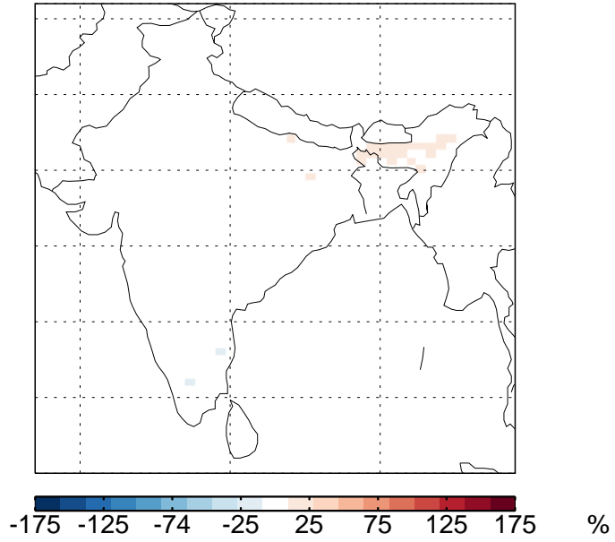
Change of Ammonium Due to Traffic: REF
