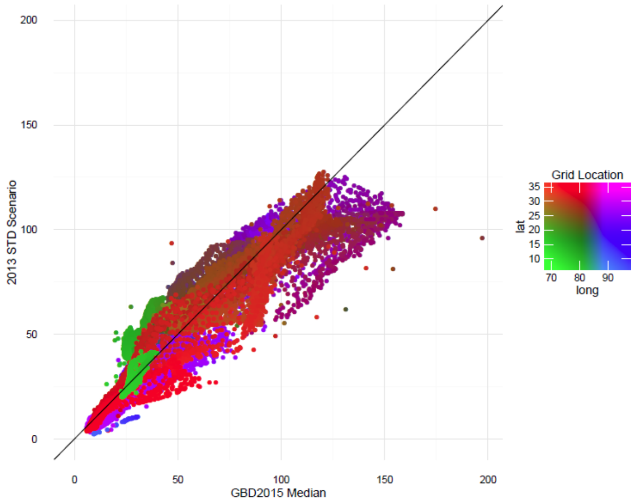
Figure A.1. Spatial Agreement between simulated ambient PM 2.5 concentrations and those estimated for GBD 2015.
