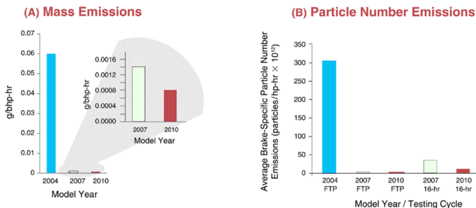
Figure 3. Substantial reductions in particle mass and number (ultrafine) emissions since 2004
